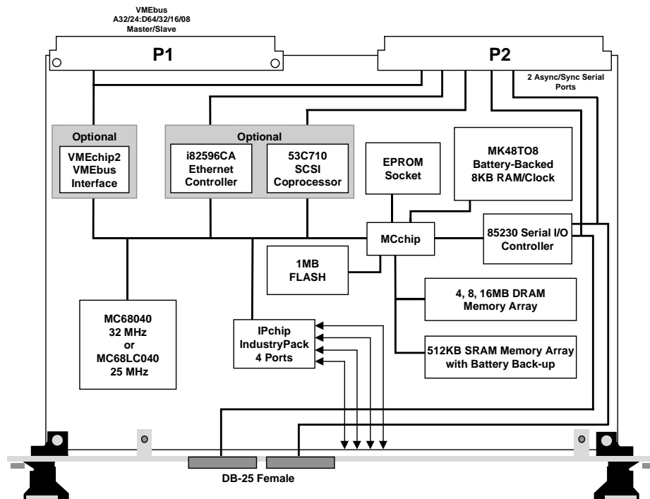
MVME162FX Embedded Controller
